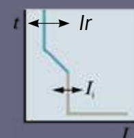
3VA1...-EF32-0AA0
